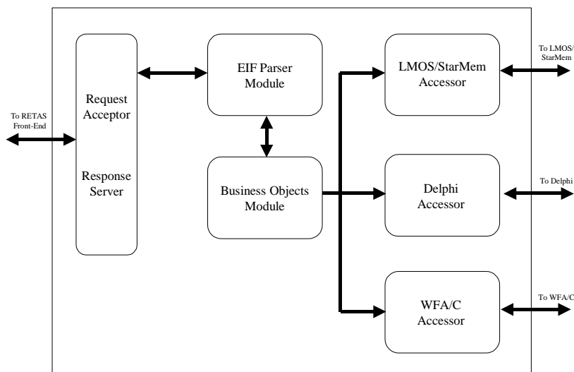
Figure 5-2: RETAS Architecture 85
